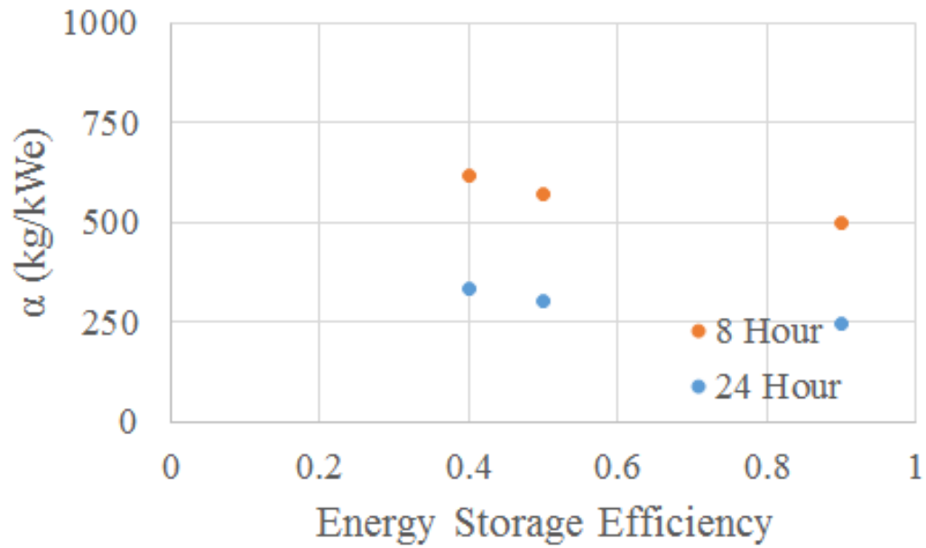
Figure 22: Sensitivities of \alpha for 8 hour and 24 hour operation to \eta_{storage} .
