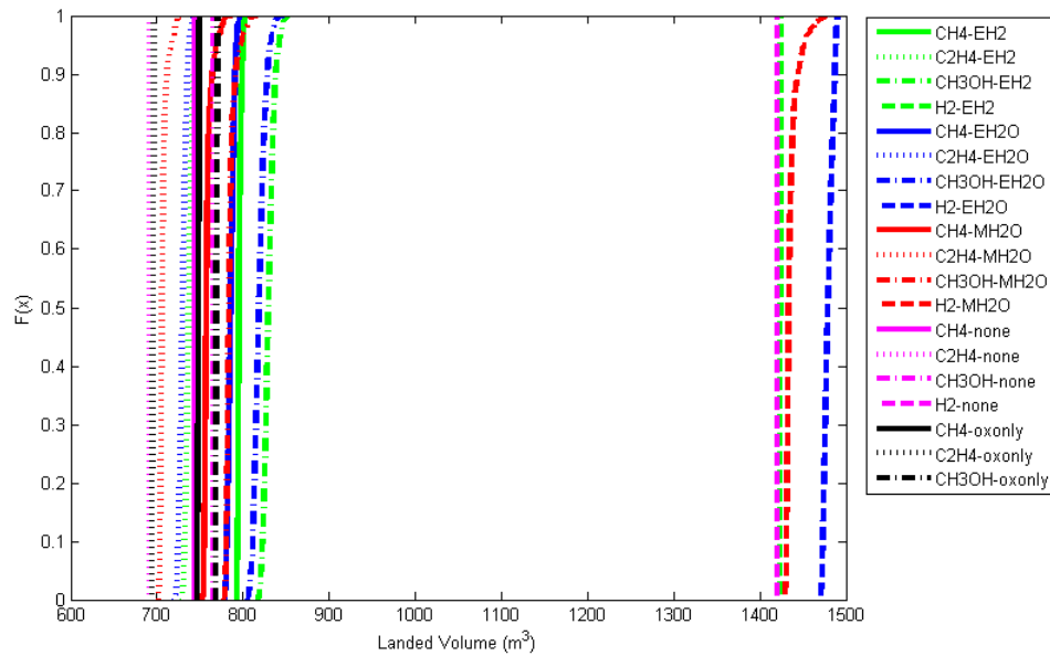
Figure 108: The landed volume (ISPP system, surface power system, and MAV) of the nineteen architectures with low launch costs and low specific mass power system.
