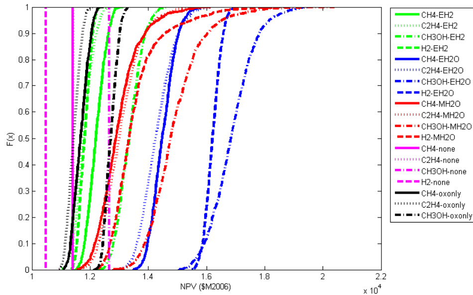
Figure 118: The net present value of the life cycle cost of the nineteen architectures with high launch costs and high specific mass power system.
